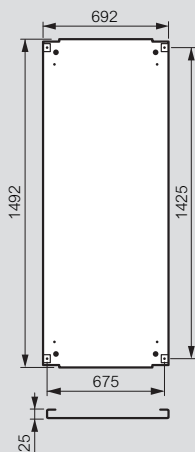
Piastra piena art. 0 349 50
