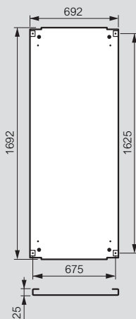
Piastra piena art. 0 344 18
