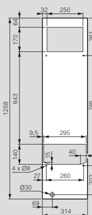
Art. 0 353 74
